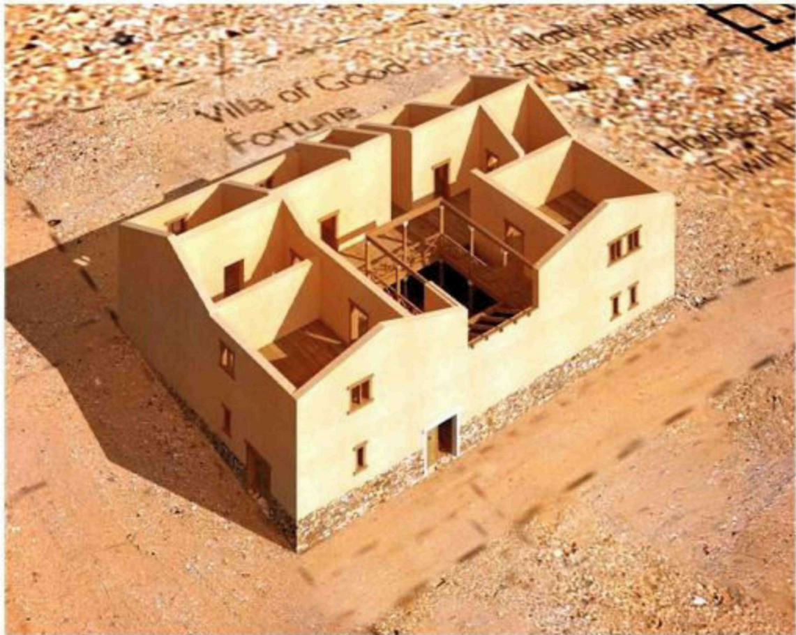
Villa of Good Fortune in ancient Olynthos. The walls of the first floor were entirely made of raw earth. The columns supporting the portico surrounding the court and its roof were made of wood.
