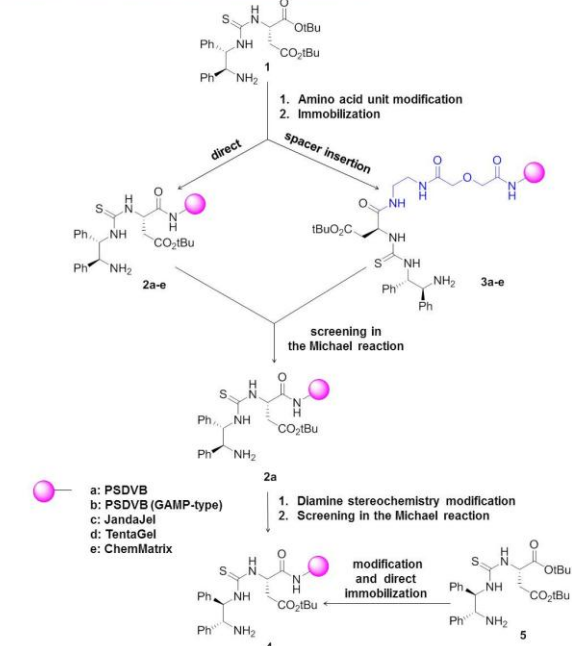
Scheme 1. Optimization of polymer-supported primary amine-thiourea catalysts based on tert -butyl aspartate and 1,2-diphenylethylenediamine.
